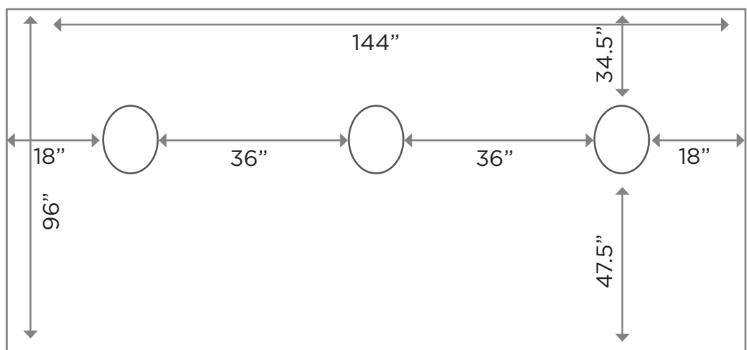
Front Panel
